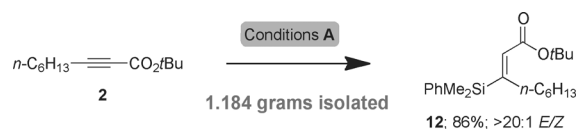
Scheme 4. Gram-scale silylation.
